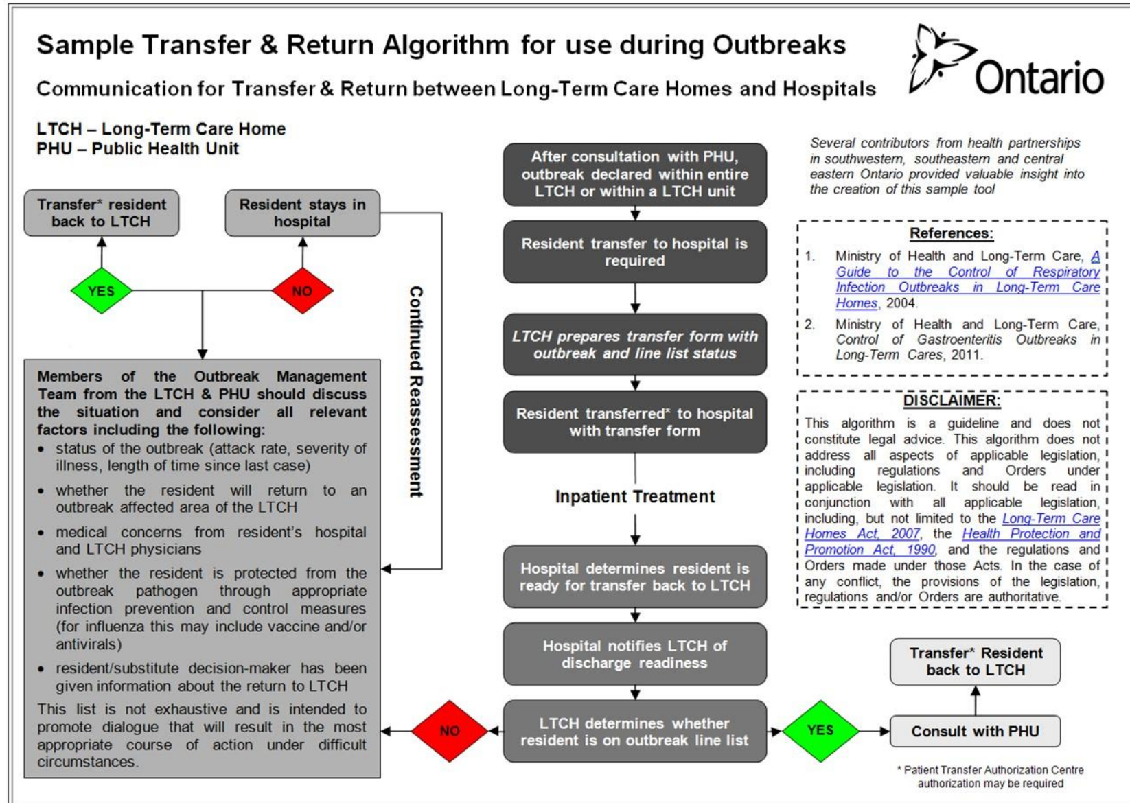
Image 9. Sample Transfer and Return Algorithm During Outbreaks (2)
